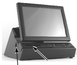
Printer cover release button Paper Exit
