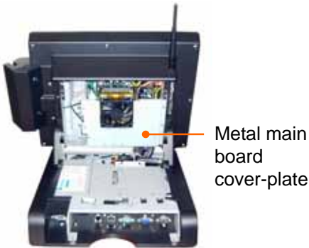
FIGURE 2-6: Q-POS REAR SYSTEM PANEL, WITH CPU AND FAN INSTALLED
