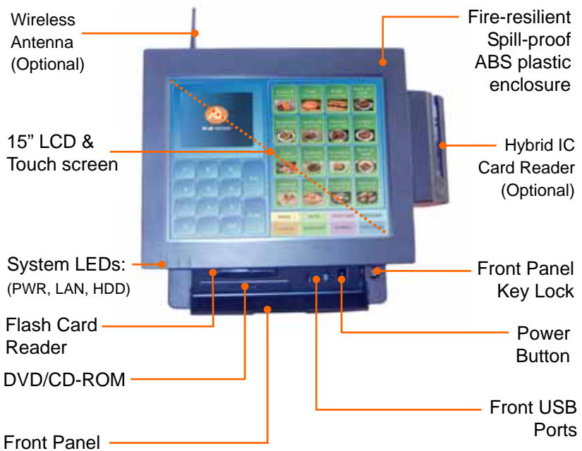
FIGURE 2-1: Q-POS FRONT VIEW
