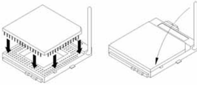
FIGURE 2-8: CPU INSTALLATION
