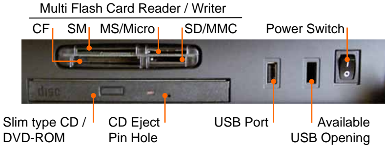
FIGURE 2-2: Q-POS FRONT PANEL
