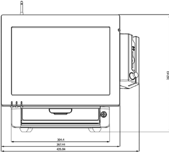
FIGURE 1-1: Q-POS FRONT VIEW DIMENSIONS (WITH OPTIONAL HYBRID CARD READER ON FRONT RIGHT SIDE)
