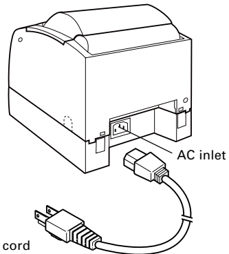
Built-in Power Supply Type
